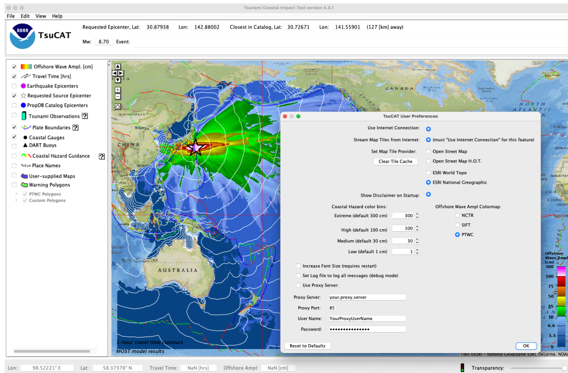
Figure 15. TsuCAT User Preferences window allowing user to customize “Coastal Hazard color bins,” select Wave Amplitude color map, and select Internet map streaming using “View->Stream Map Tiles from Internet.”
