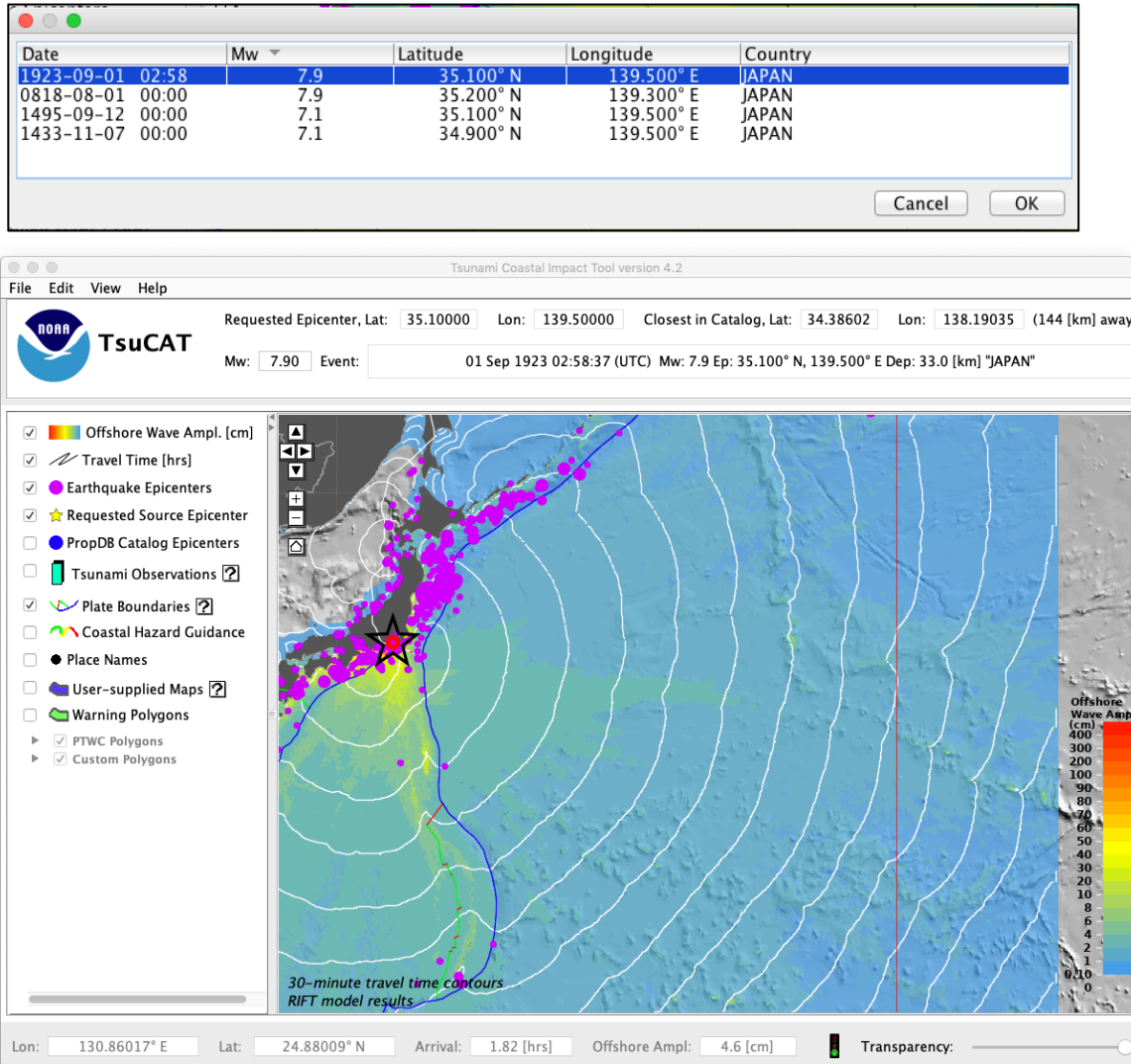
Figure 7: Historical tsunamigenic earthquakes (purple dots) from the Global Historical Tsunami Database
