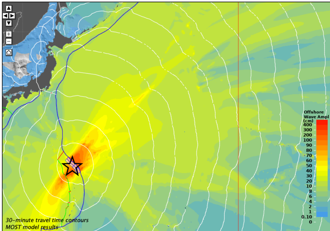
Figure 6: Arbitrary Mw=8.6 along the Kamchatkai-Yap subduction zone.
