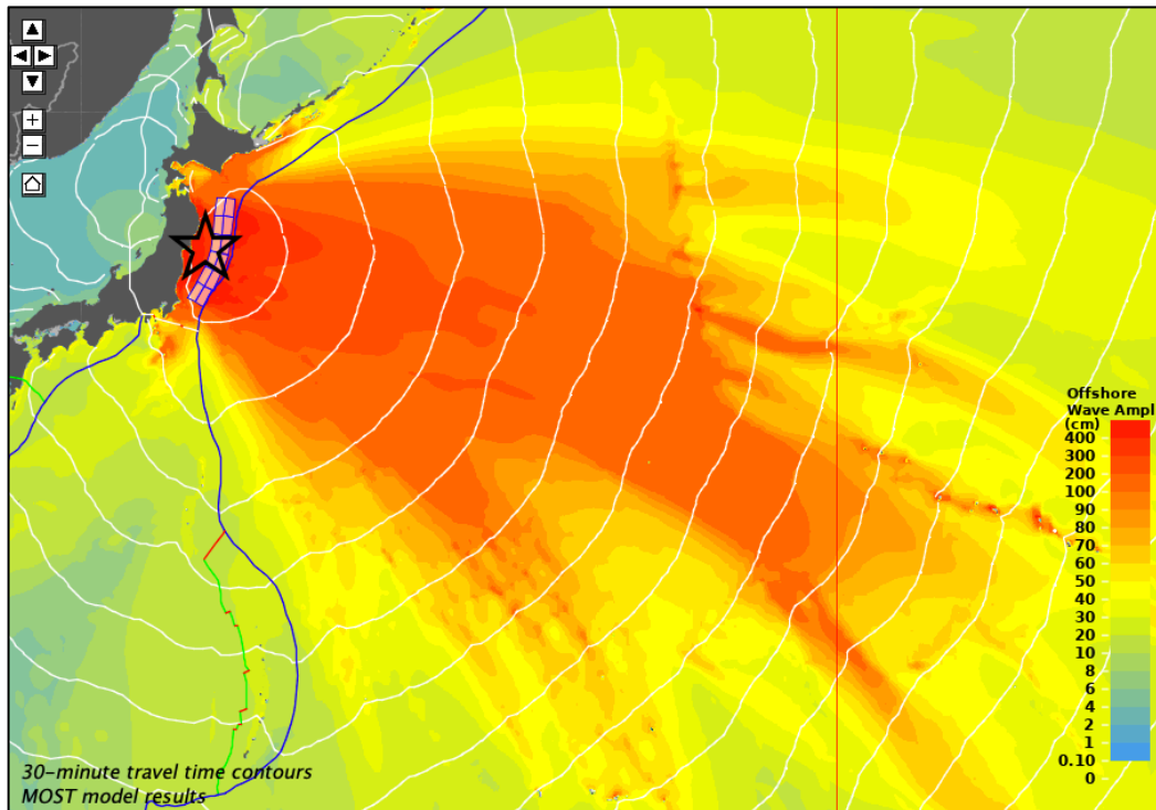
Figure 3: The Propagation Database unit sources selected for the Great Japan tsunami of 2011.
