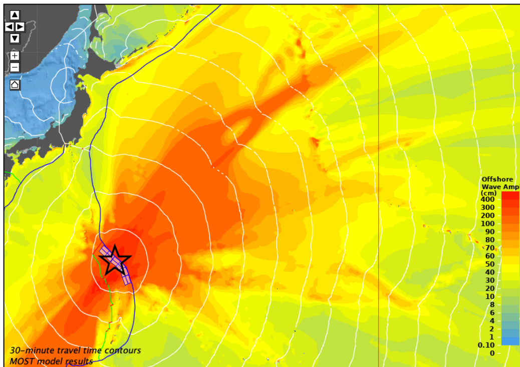
Figure 5: An arbitrary M_w=9.1 along the Kamchatkai-Yap (ki) subduction zone.
