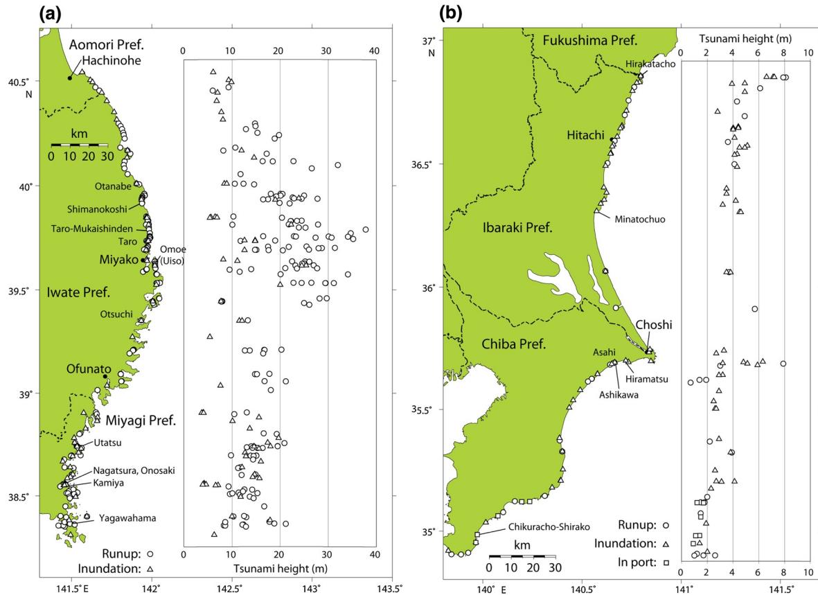
a Distribution of tsunami heights in Aomori, Iwate, and Miyagi prefectures (TSUJI et al. 2011). Circles and triangles indicate runup and inundation heights, respectively. The dashed lines indicate prefectural boundaries. b Distribution of tsunami heights in Ibaraki and Chiba prefectures. Circles, triangles, and squares indicate runup heights, inundation heights, and tsunami heights in ports, respectively
