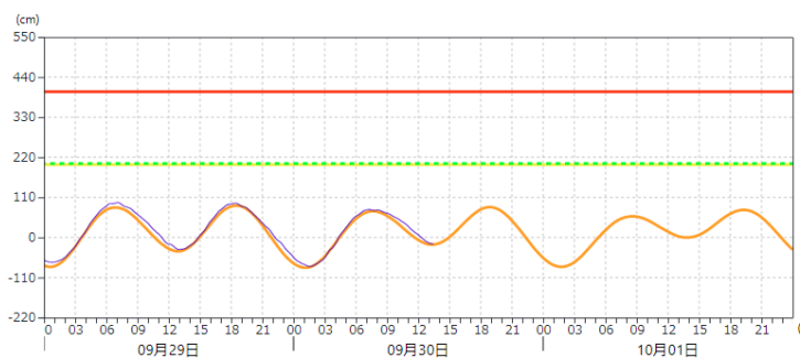
Fig. 3: Tokyo sea level observations for September 29 – October 1, 2022.
