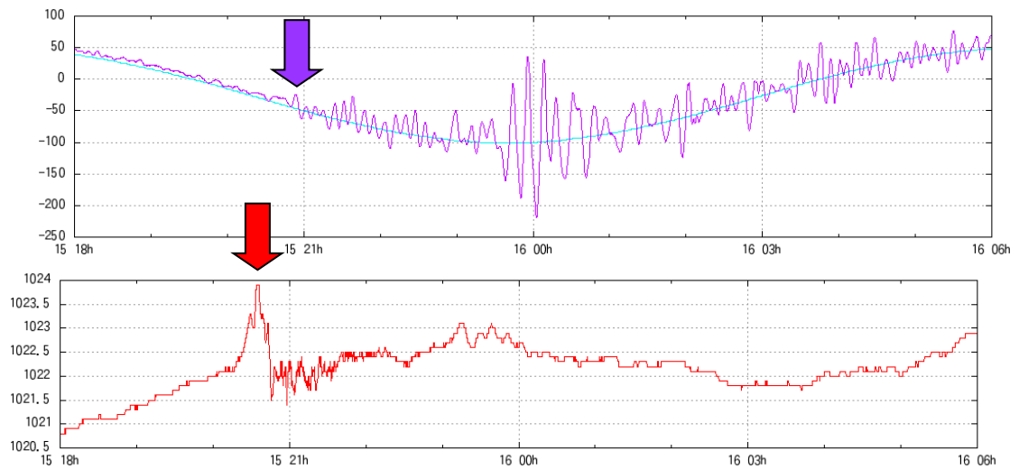
Fig.8: Tide level changes in Amami due to the Tonga volcanic eruption (upper panel unit:cm) and pressure changes (lower panel, unit:hPa). The tide level change (purple arrow) occurred about 30~60 minutes after the pressure change of about 2 hPa (red arrow).
