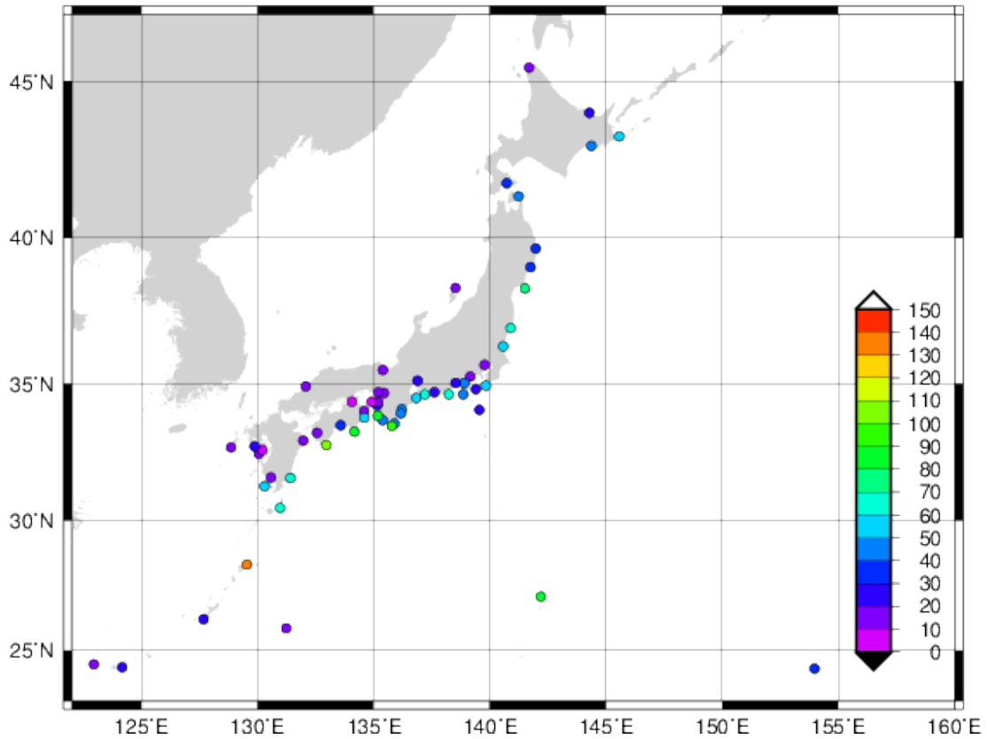
Fig.7: Maximum wave heights on the tide gauge in japan(unit:cm).
